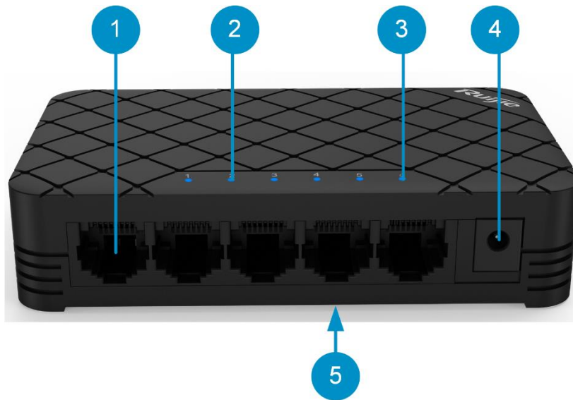
Figure 1-6 Front Panel of RG-ES05G
