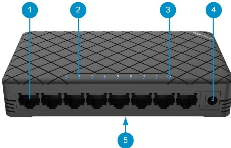
Figure 1-8 Front Panel of RG-ES08G
