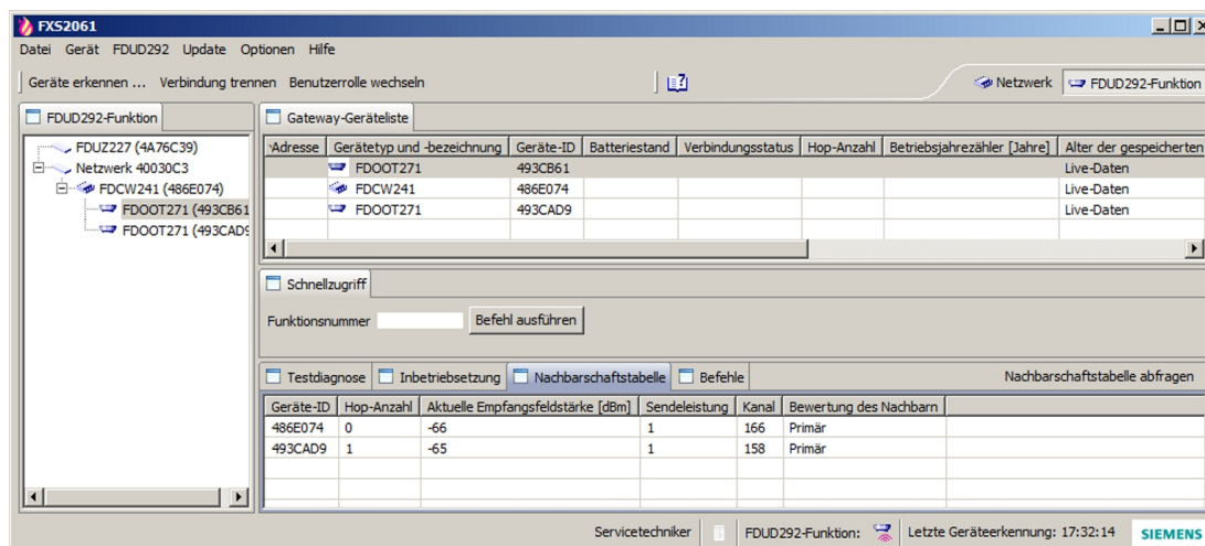
Fig. 1: Overview of the program window FXS2061 SWING tool
