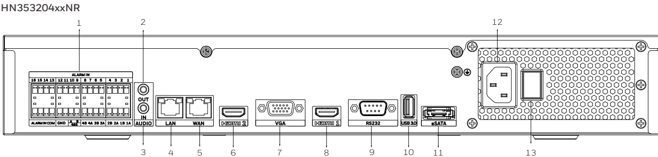
1. Alarm Input/Output 2. Audio Out 3. Audio In 4. LAN Port 5. WAN Port 6. HDMI 2 Port 7. VGA Port 8. HDMI 1 Port 9. RS232 Port 10. USB Port 11. eSATA Port 12. Power Input 13. Power Switch
