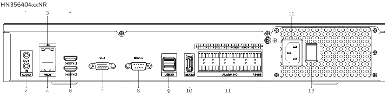
1. Audio Out 2. Audio In 3. LAN Port 4. WAN Port 5. HDMI 1 Port 6. HDMI 2 Port 7. VGA Port 8. RS232 Port 9. USB Port 10. eSATA Port 11. Alarm Input/Output 12. Power Input 13. Power Switch
