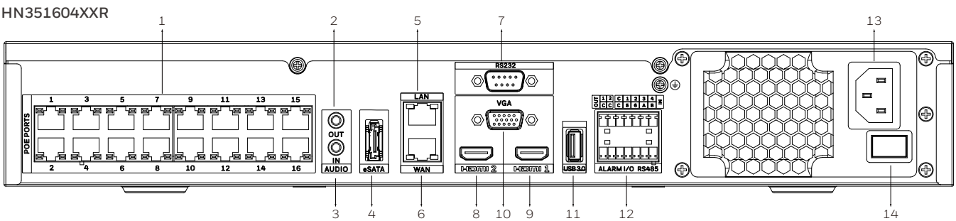
1. PoE Ports 2. Audio Out 3. Audio In 4. eSATA Port 5. LAN Port 6. WAN Port 7. RS232 Port 8. HDMI 2 Port 9. HDMI 1 Port 10. VGA Port 11. USB Port 12. Alarm Input/Output 13. Power Input 14. Power Switch
