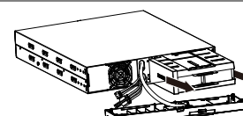
Battery Set with 10x 12V/9Ah batteries (Plug-and-Play solution incl. case and cabling to change internal bat. Set of VFI 10000 P/RT LCD) Datasheet: Link
